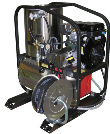
Short Skid
